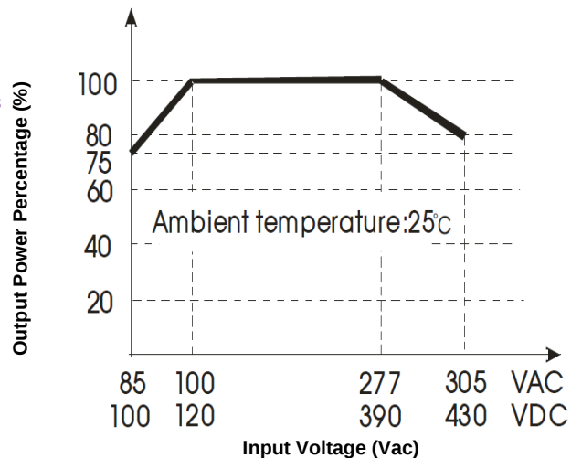
Figure 2. Input Voltage Derating Curve
